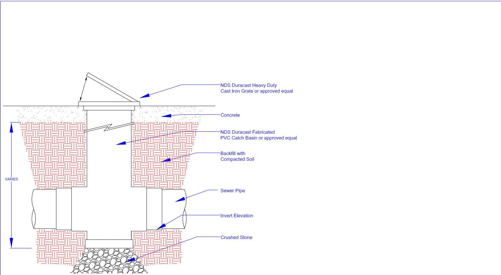
NDS DURACAST SQUARE HINGED GRATE (P/N D12) WITH NDS DURACAST PVC CATCH BASIN CONNECTED TO A SEWER & DRAIN PIPE
